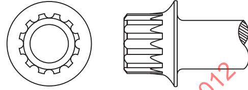
12-Spline Head
