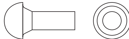
Swell-Neck Rivet
