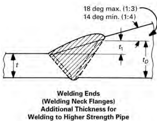
Figure 1 Bevel for Outside Thickness
