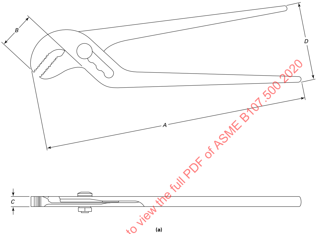
Figure 13.1.2-1 Category 23 Type I, Class 2, Adjustable Joint, Angle Nose, Multiple Holes
